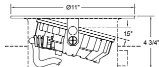
Niche Mounted
