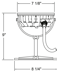
Pedestal Mounted
